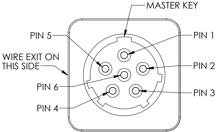
PIN LAYOUT AND ORIENTATION OF BA5590 CONNECTOR (ITEM #1)
