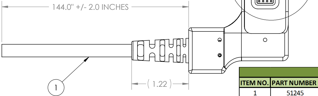
DETAIL A SCALE 2 : 1
