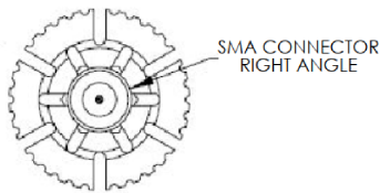
FRONT VIEW (WITH SPINNER)
