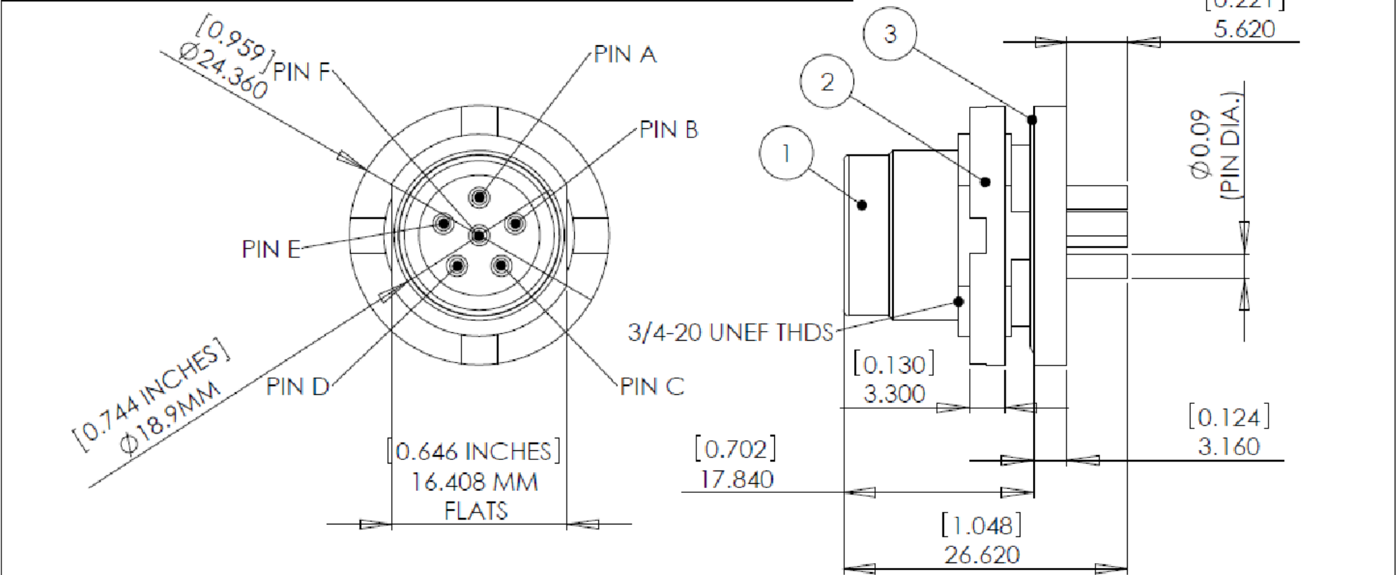
PANEL CUTOUT DIAGRAM
